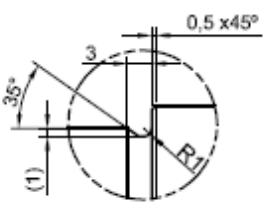
DETALLE X (2.5:1)
